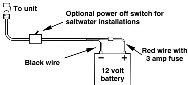
Power connections for the IntelliMap 502C GPS unit.
